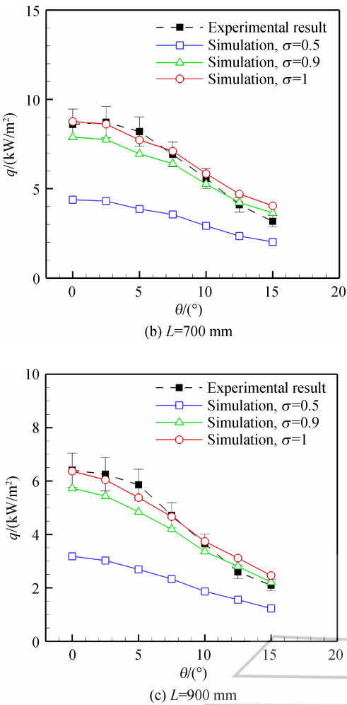
图 8 计算得到的热流密度和实验结果的对比 Fig. 8 Comparison between simulation results and experimental results of heat flux density
